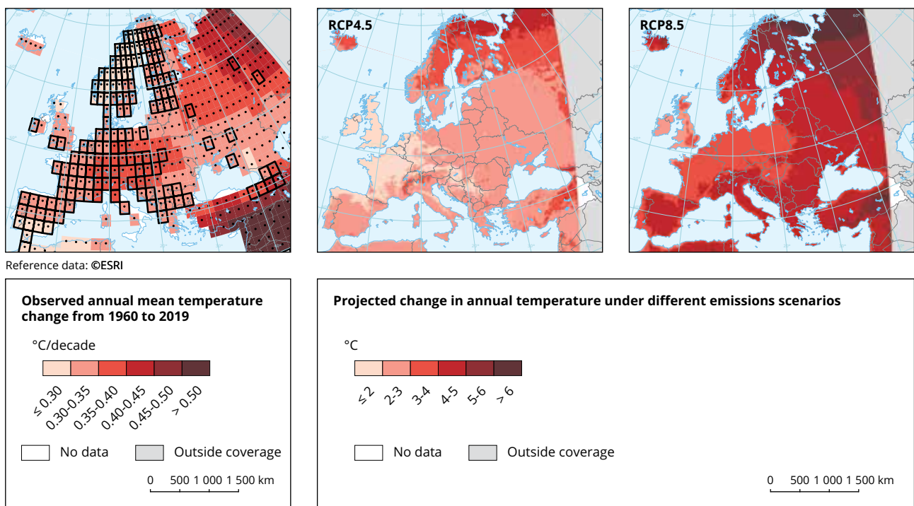
Map 3.1 Observed annual mean temperature change from 1960 to 2019 (left panel) and projected change under different emissions scenarios (right panels) in Europe
