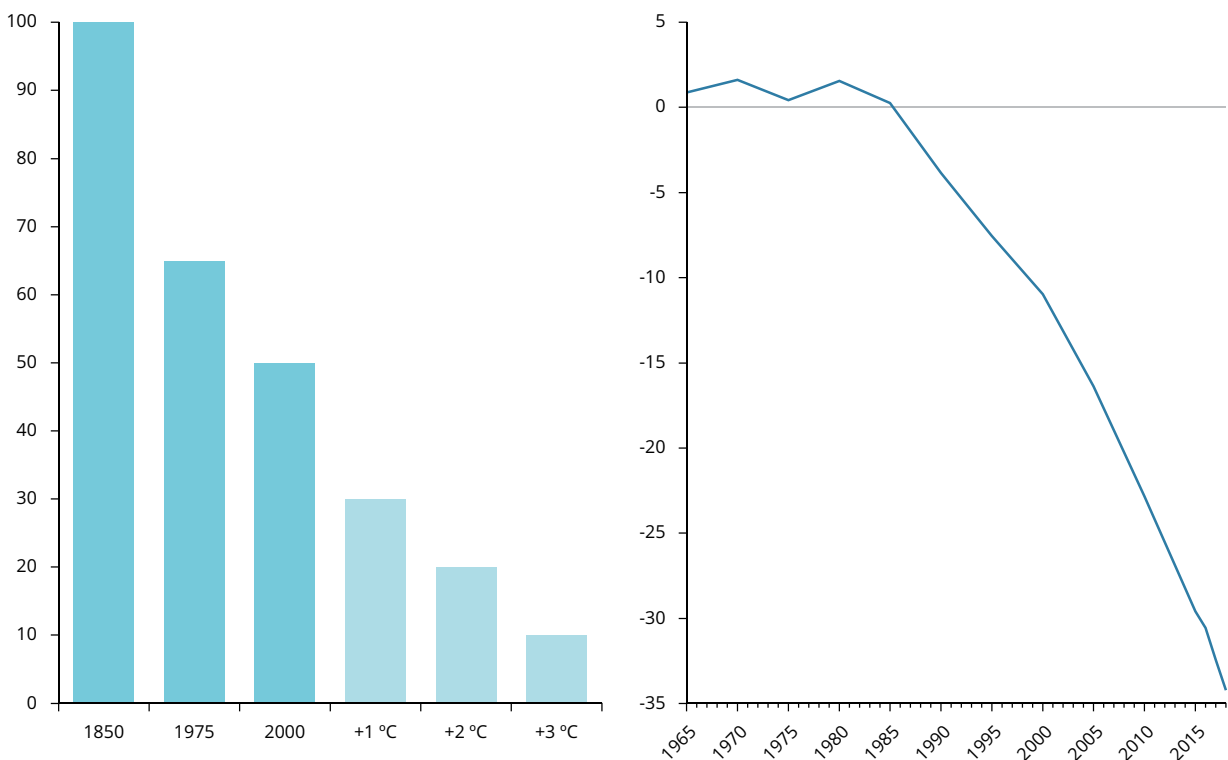
Figure 3.2 Remaining glacier surface in the Alps (left); annual cumulative glacier mass balance in Switzerland (right)
