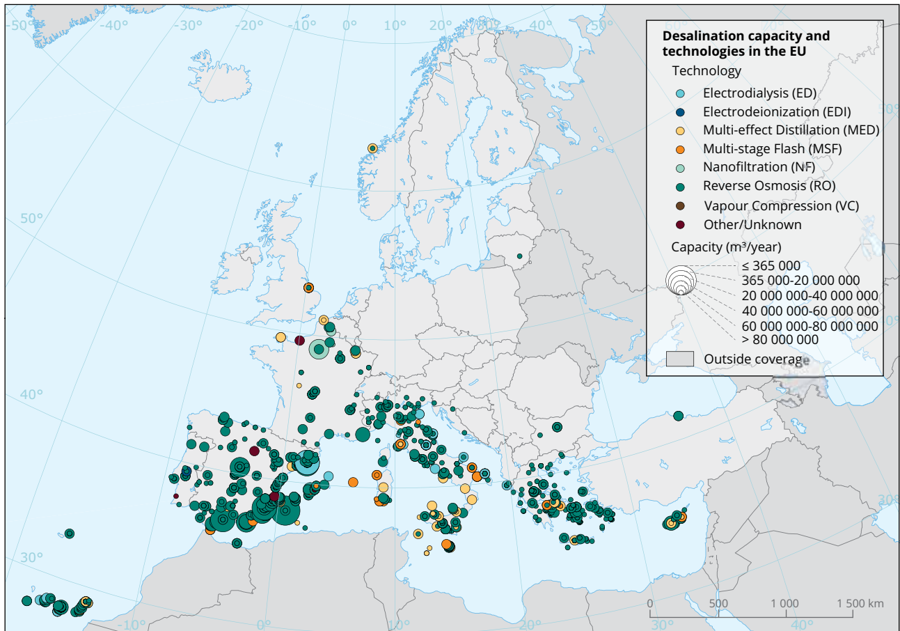
Map 6.1 Desalination capacity and technologies in the EU
