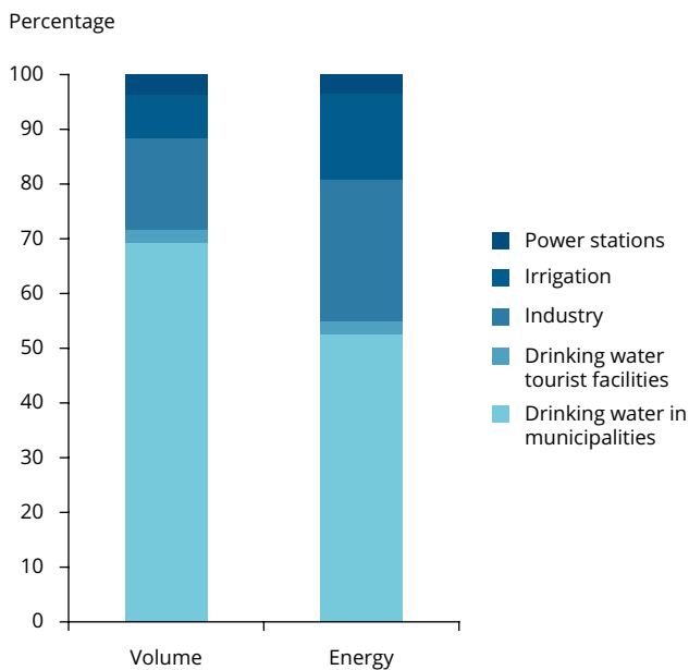
Figure 6.2 Volume supplied and energy used during desalination of water for various end users
