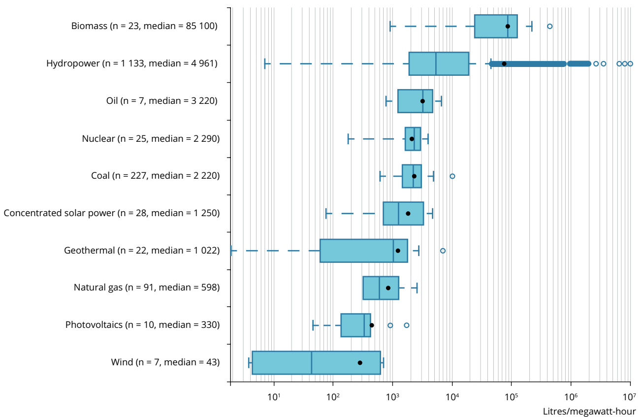
Figure 4.11 Water consumption per unit of energy generated during the life cycle of different types of energy sources
