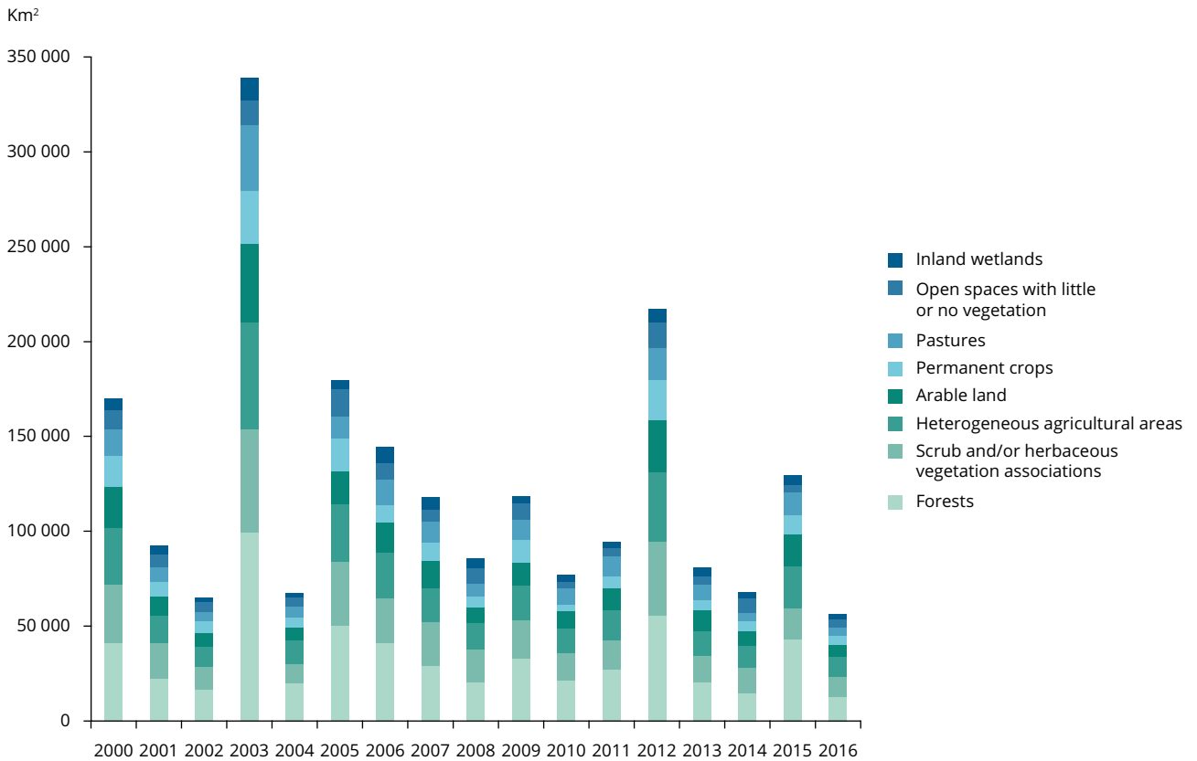
Figure 1.1 Area affected by reduced vegetation productivity due to water deficit, by land use type in Europe, 2000-2016
