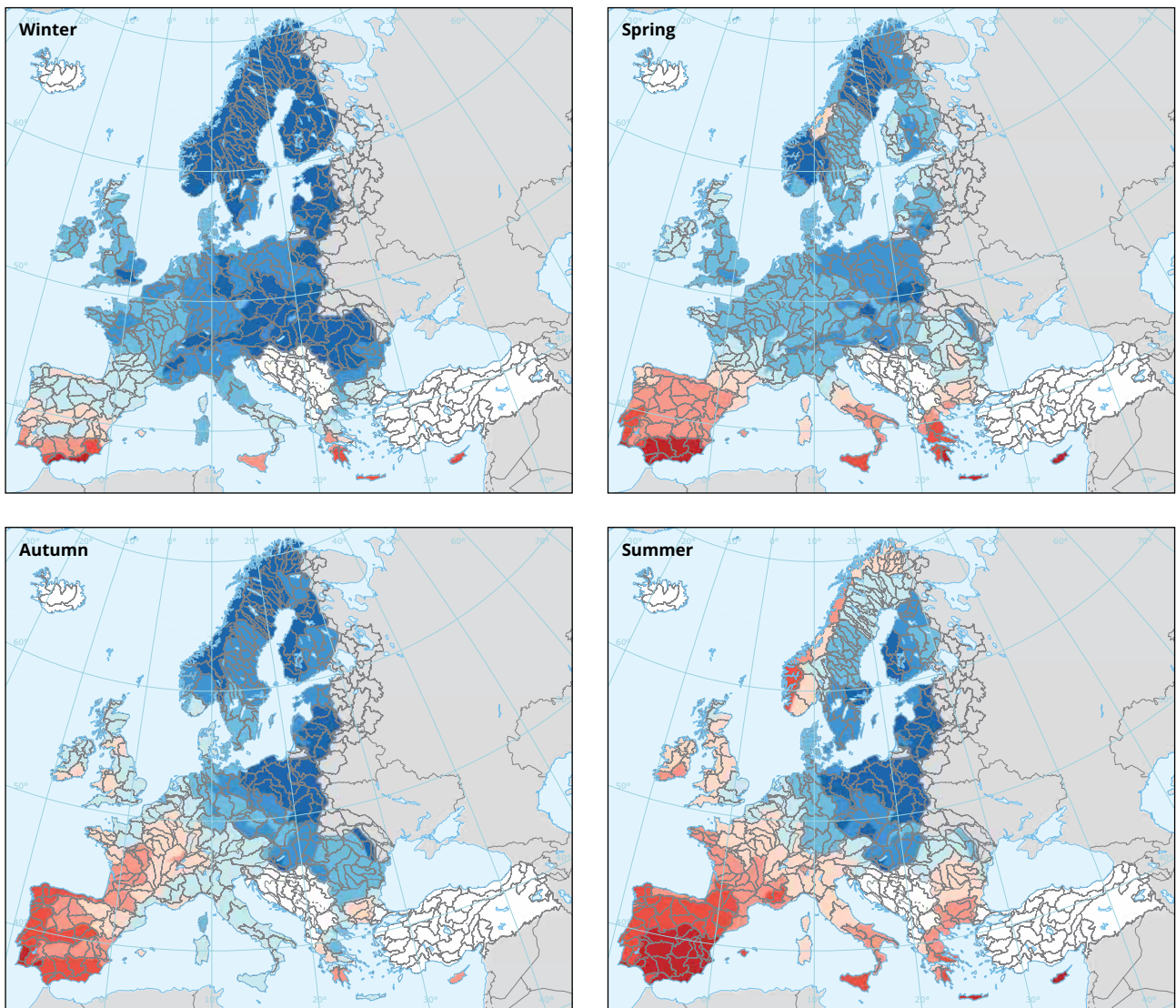
Map 3.10 Projected percentage seasonal change in river discharge (clockwise from upper left: Season 1, Season 2, Season 3, Season 4) for a 3 °C temperature scenario
