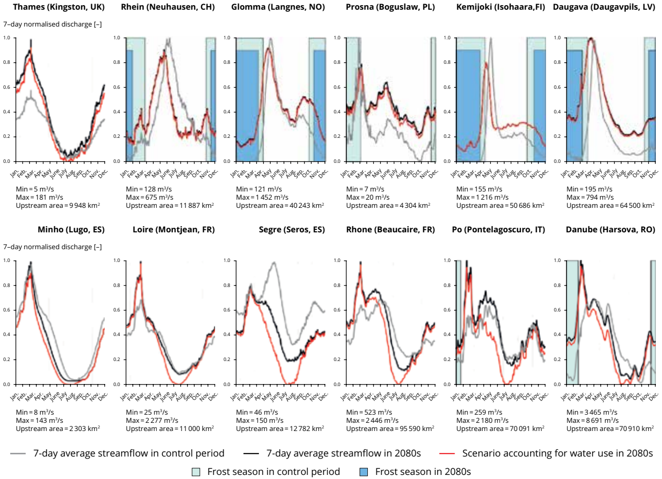
Figure 3.4 Projected change in seasonal streamflow for 12 European rivers
