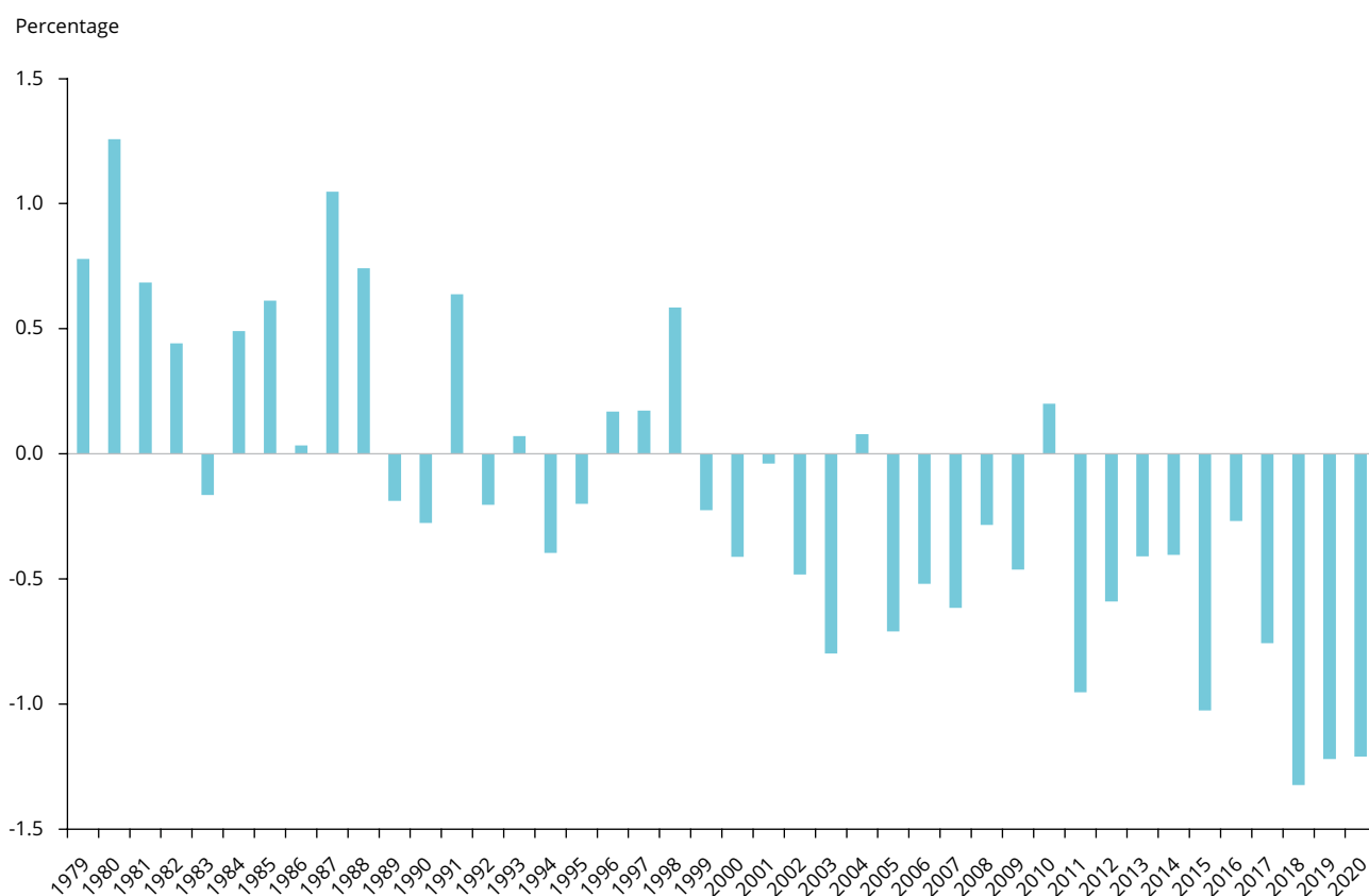
Figure 3.3 Annual soil moisture anomalies in Europe between 1979 and 2020
