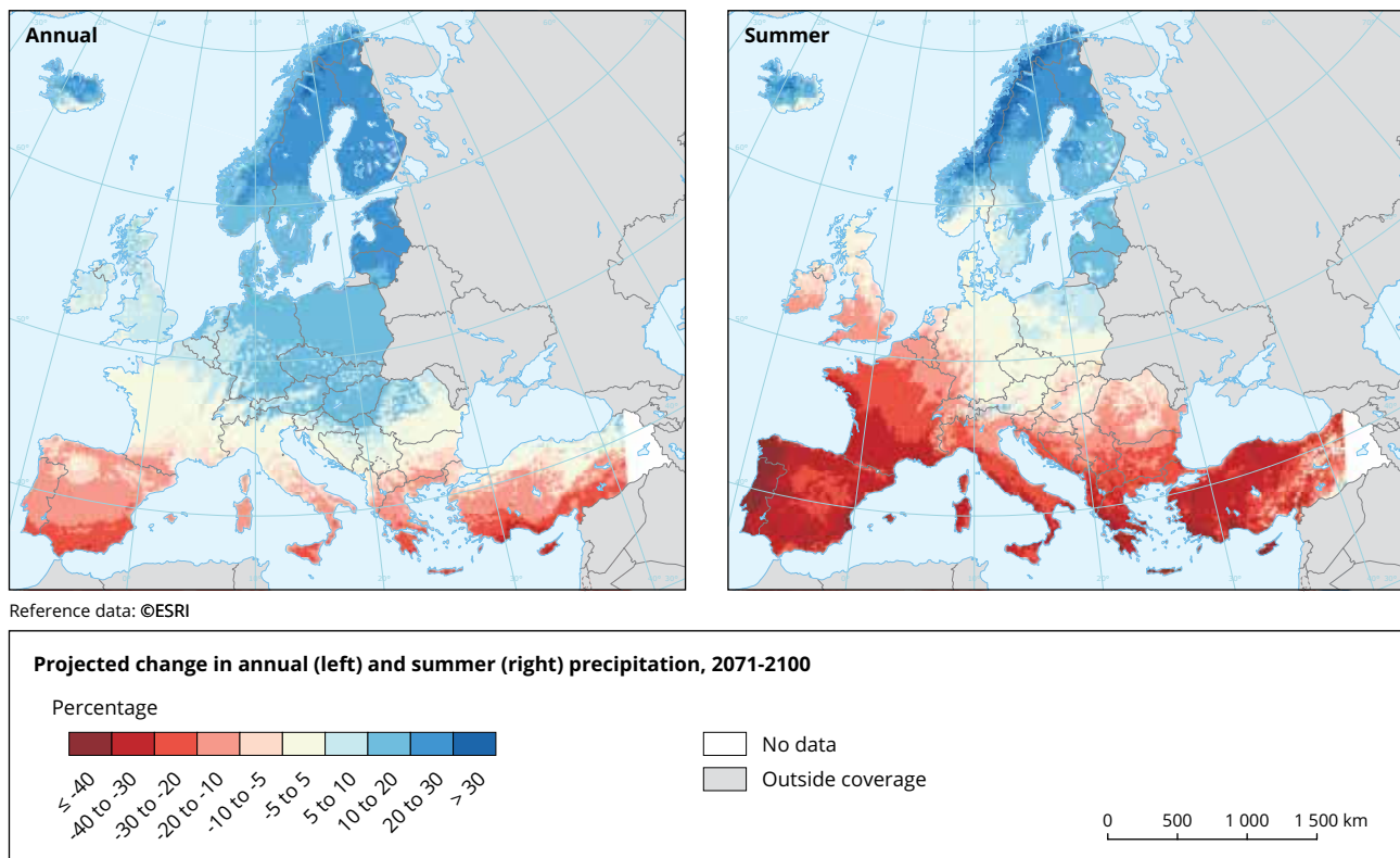
Map 3.3 Projected change in annual (left) and summer (right) precipitation across Europe for the period 2071-2100 (versus 1971-2000 average)
