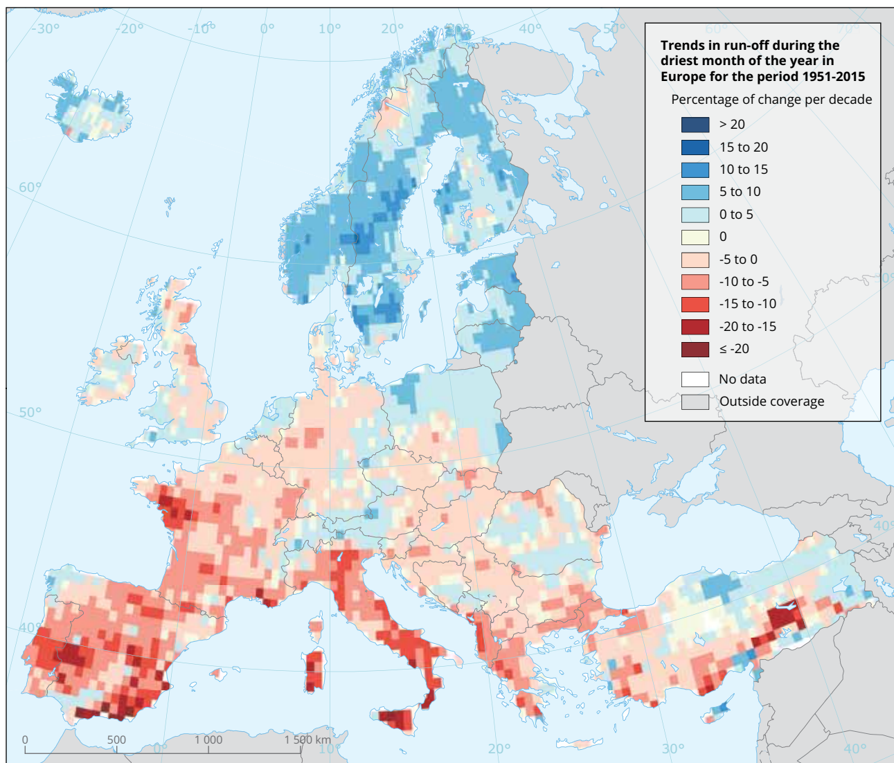
Map 3.9 Trends in run-off during the driest month of the year in Europe for the period 1951-2015
