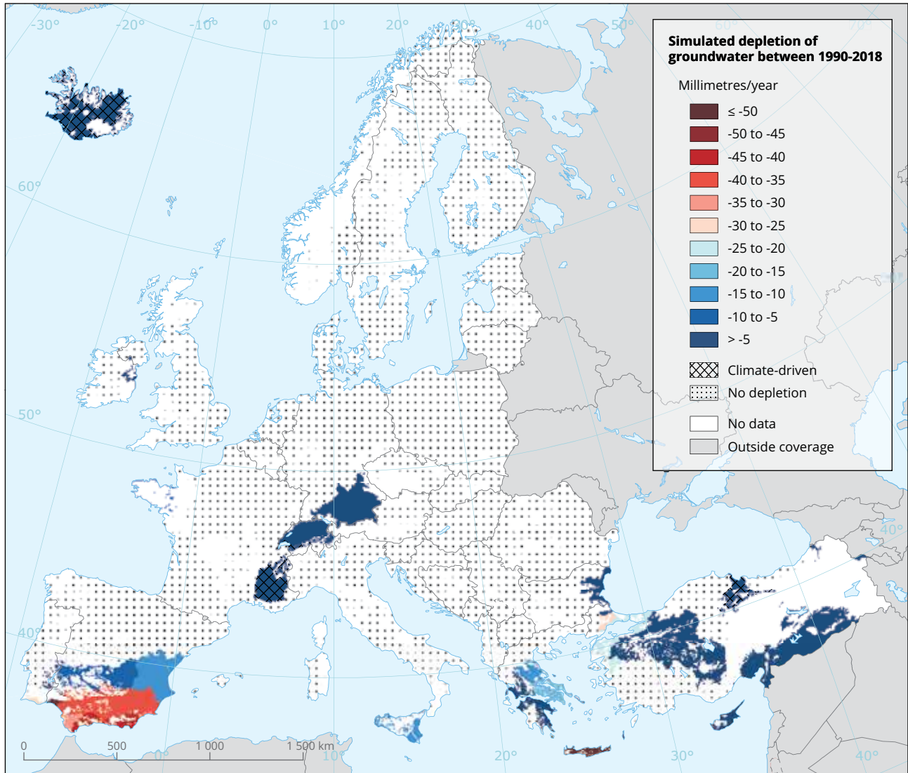
Map 1.1 Simulated depletion of groundwater (mm per year) between 1990 and 2018
