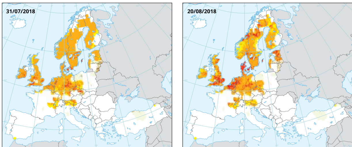
Map 1.2 The Combined Drought Indicator for the last 10-day period of July 2018 (left) and the second 10-day period of August 2018 (right)
