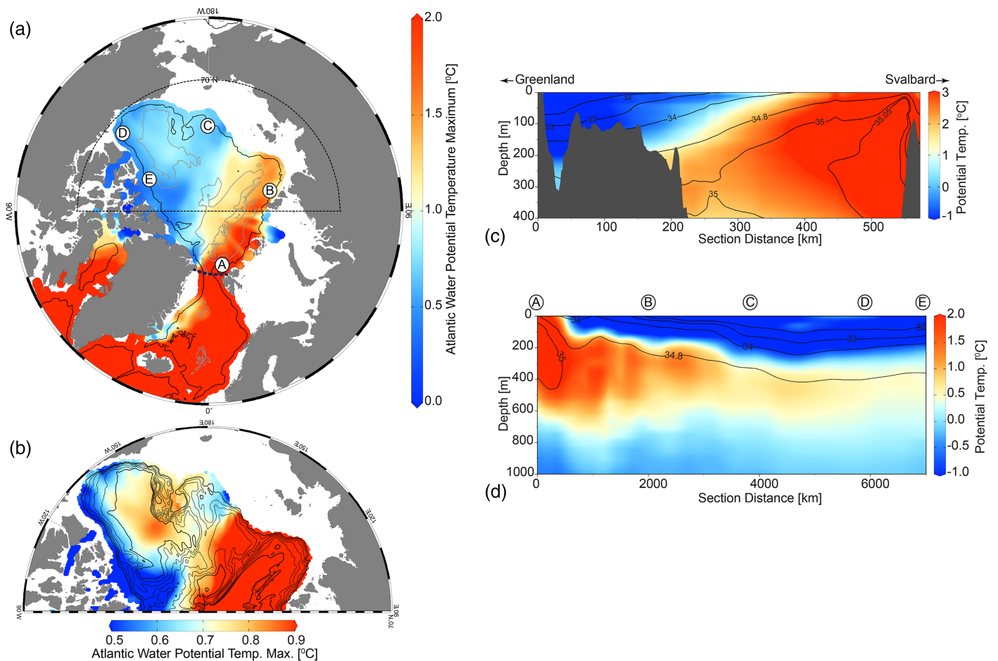
Figure 5. Maps of Atlantic Water potential temperature maximum ( ^{\circ}\text{C} ) for (a) the Arctic Ocean and (b) the sector bounded by the thin dotted black lines in (a). Bathymetric contours in (b) are in intervals of 500 m; the deepest contour shown is 3,500 m. Sections of potential temperature ( ^{\circ}\text{C} , colors) and salinity (contours) (c) across Fram Strait from west to east along 80^{\circ}\text{N} (thick dotted line shown in panel (a)); cooler, fresher water in the west flows south, while the warmer, saltier water to the east flows north, entering the Arctic Ocean from the Nordic Seas) and (d) along the 1,000-m isobath moving cyclonically around the Arctic basin with letters A–E corresponding to their locations marked in panel (a). Data are from WOD18, 2005–2017.
