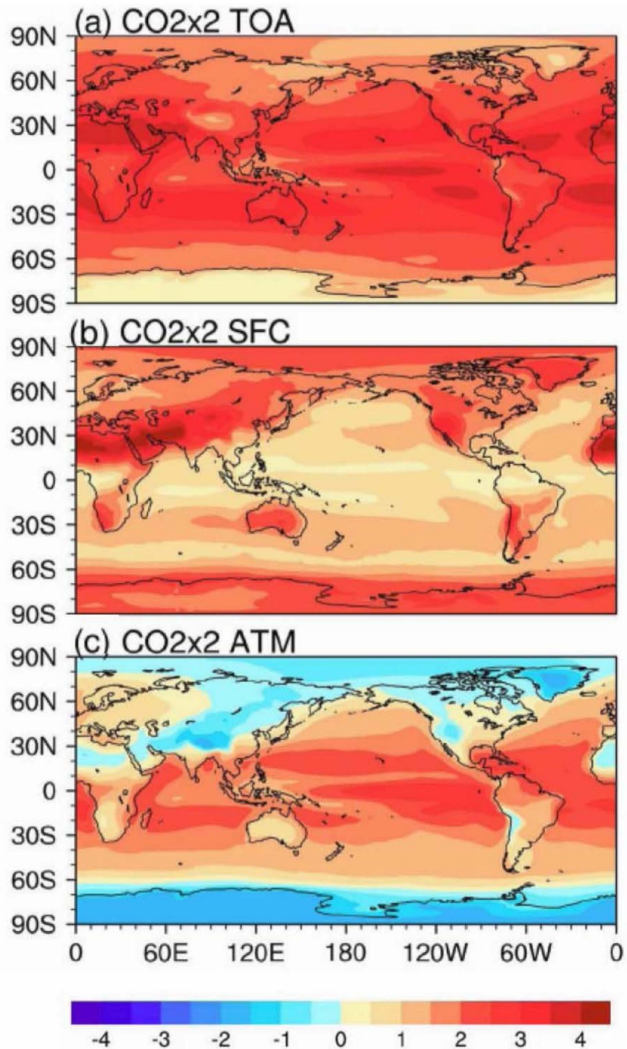
Figure 3. Instantaneous radiative forcing (in \text{W m}^{-2} ) from doubling \text{CO}_2 as calculated by the rapid radiative transfer model (RRTM). The forcing is defined as the change in the net (i.e. longwave plus shortwave) downward radiative flux, and is shown for: (a) the top-of-atmosphere (TOA); (b) the surface (SFC); and (c) the atmospheric column (ATM, defined as TOA minus SFC). Adapted with permission from Huang et al (2017). © 2017. American Geophysical Union. All Rights Reserved.
