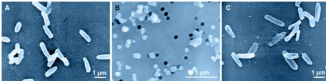
Morphological characteristics of Vibrio harveyi SF1 analyzed with a scanning electron microscope.
