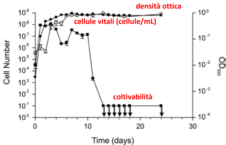
Fig. 3. The viability (cells/mL) (●), optical density (○) and culturability (cfu/mL) (■) of H. pylori cells aged in laboratory culture . Error bars represent the SEM of duplicate samples and ↓ indicate culturability below the limit of detection. Taken from Adams et al. , 2003.
