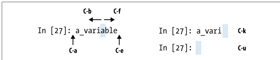
Figure 3-1. Illustration of some of IPython's keyboard shortcuts
