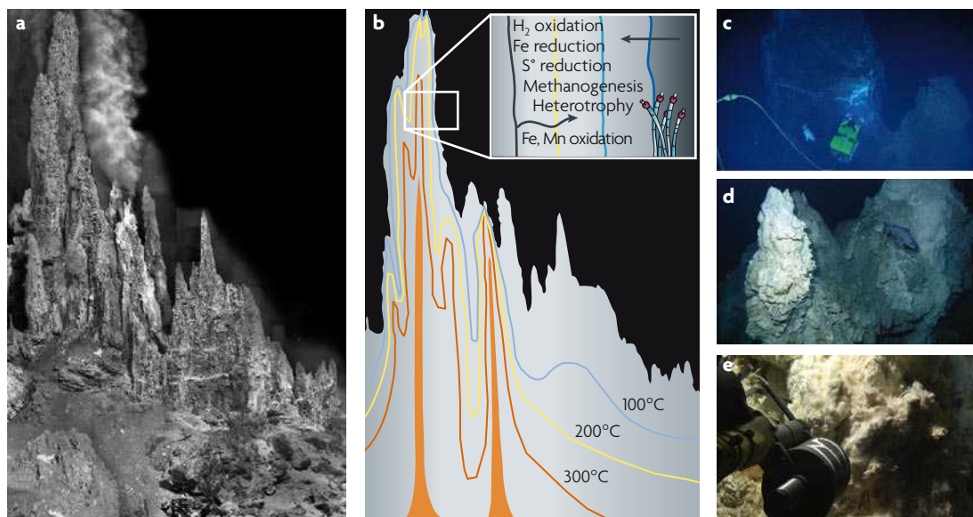
Figure 2 | Hydrothermal vents. There are two main types of hydrothermal vent: the black smoker type ( a,b ) and the Lost City type ( c–e ). a | A black smoker in the Faulty Towers complex in the Mofra hydrothermal field on the Endeavour Segment of the Juan de Fuca Ridge. The tallest chimney rises 22 metres above the sea-floor. The 'furry' appearance of the chimneys reflects the fact that the chimney walls are encrusted in dense communities of tube worms, scale worms, palm worms, sulphide worms and limpets. The two-pronged chimney in the middle with an active plume is a 300°C chimney called Finn, from which a 121°C organism was cultured that uses Fe(III) as an electron acceptor in the presence of N_2 and CO_2 (REF. 15). b | The outer surface of black smoker chimneys is bathed in a mixture of 2°C, oxygenated sea-water and warm vent fluid that escapes from within the structure. The inner walls that form the boundary of the central up-flow conduits commonly exceed 300°C, and temperatures are fixed by a steady supply of rapidly rising, strongly reducing vent fluid. Intermediate conditions exist as gradients between these extremes. Changes in microbial abundance, diversity and community structure have been associated with inferred environmental gradients in the chimney walls 99,100 . c | Microbial sampling at the Lost City hydrothermal field. The robotic vehicle Hercules is shown hovering near the summit of the 60-metres-tall Poseidon complex. White areas are active or recently active sites of venting. d | The top left part of the Nature Tower. Wreck-fish, which are ~1 metre in length and are commonly found at a water depth of 750 metres, routinely investigated the vehicles. The Poseidon complex has four pinnacles, two of which are shown here. Actively venting edifices are composed of aragonite ( CaCO_3 ) and brucite ( Mg(OH)_2 ). The grey–brown material also contains carbonate, but is richer in calcite that has recrystallized from aragonite. e | A close up of a 75°C, diffusely venting carbonate chimney showing a titanium water sampler. Dense colonies of filamentous bacteria thrive in the high pH, CH_4 - and H_2 -rich fluids. The insides of the chimneys are dominated by a single phylotype of archaea from the Methanosarcinales order that grow at 80°C. A phylotype of anaerobic methanotrophic archaea are restricted to lower-temperature chimneys. Bacterial 16S ribosomal RNA gene sequences correspond to a diverse community that includes species of Methylobacter (or Methylomonas ), species of Thiomicrospira , members of the Firmicutes phylum and Desulfotomaculum alkaliphilus 28 . Parts a,b courtesy of D. Kelley and J. Deloney, University of Washington, USA. Images c–e courtesy of D. Kelley, Institute for Exploration, University of Rhode Island, USA, and the National Ocean and Atmospheric Administration Office of Ocean Exploration.
