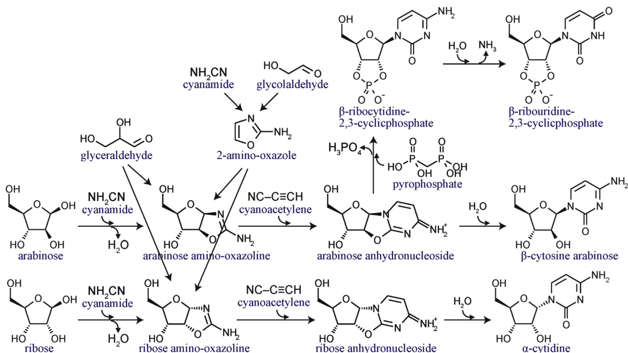
Figure 12. Reaction pathway for abiotic synthesis of pyrimidine nucleotides.
